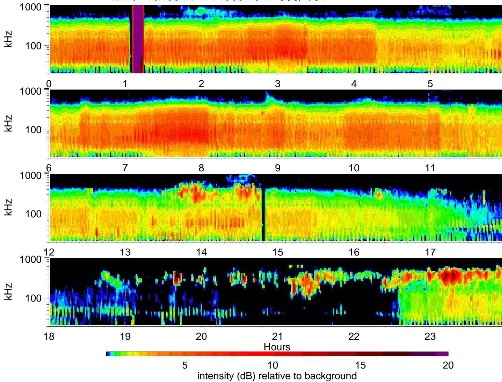
Wind Waves RAD1 receiver: 2006/7/31
