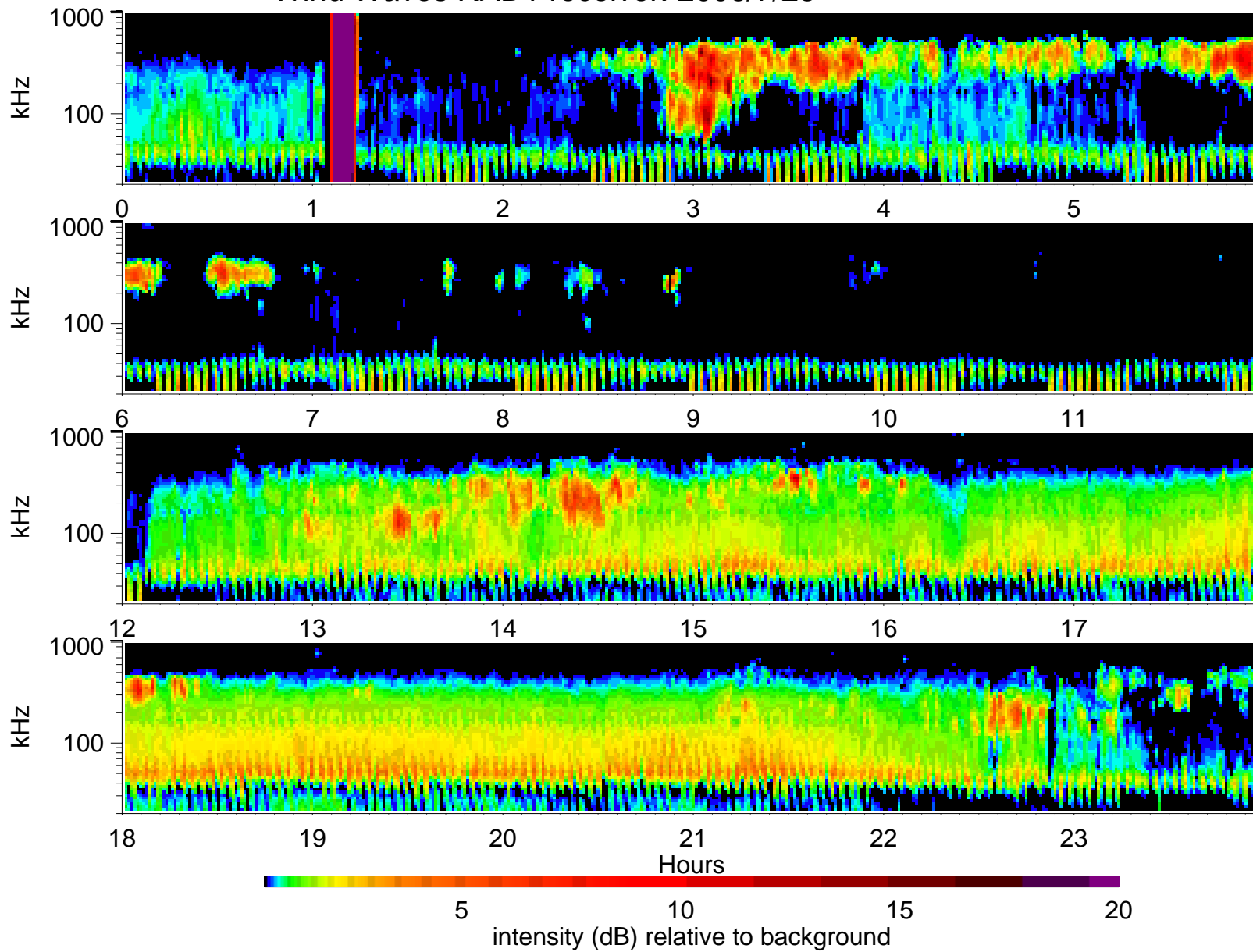
Wind Waves RAD1 receiver: 2006/7/25
