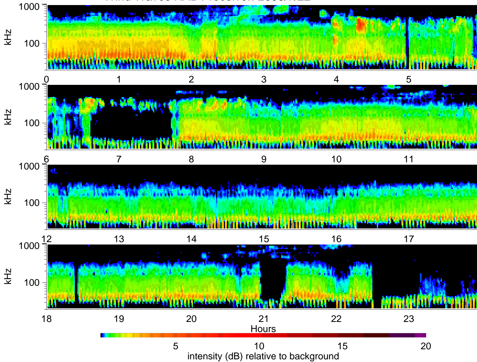
Wind Waves RAD1 receiver: 2006/7/22
