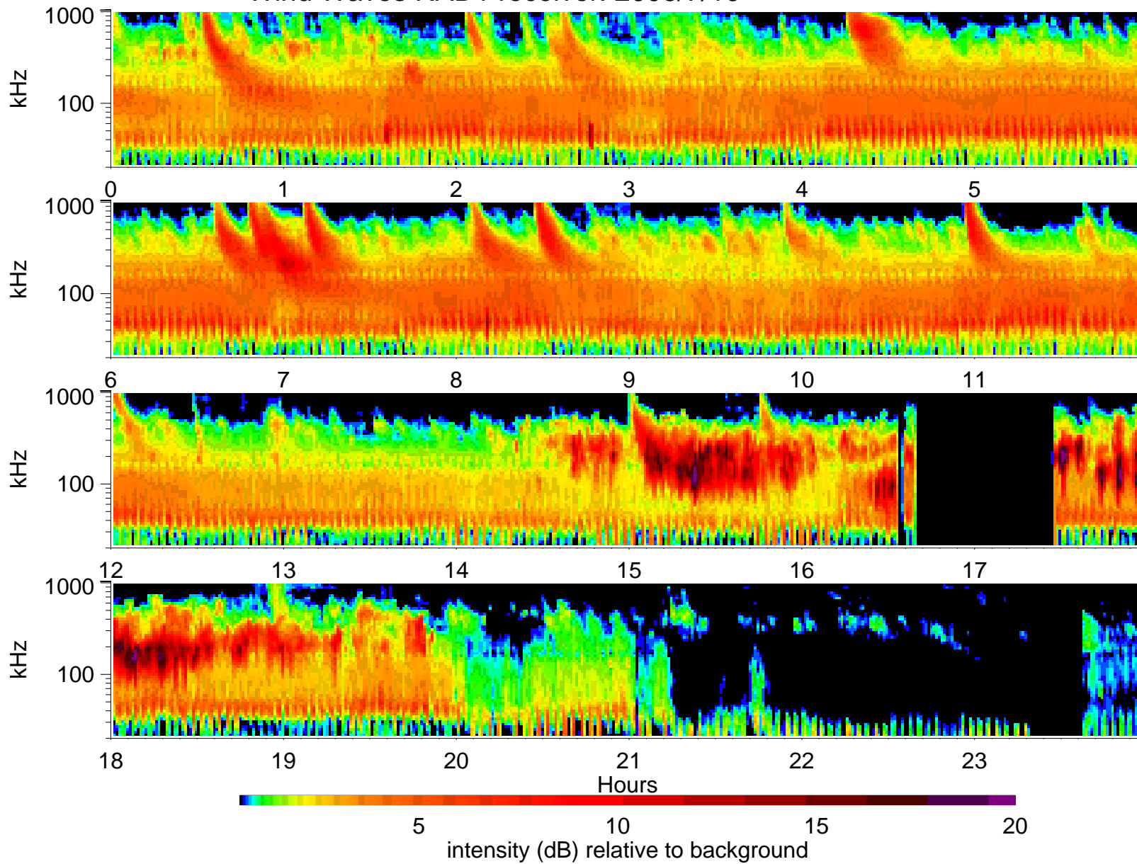
Wind Waves RAD1 receiver: 2006/7/10
