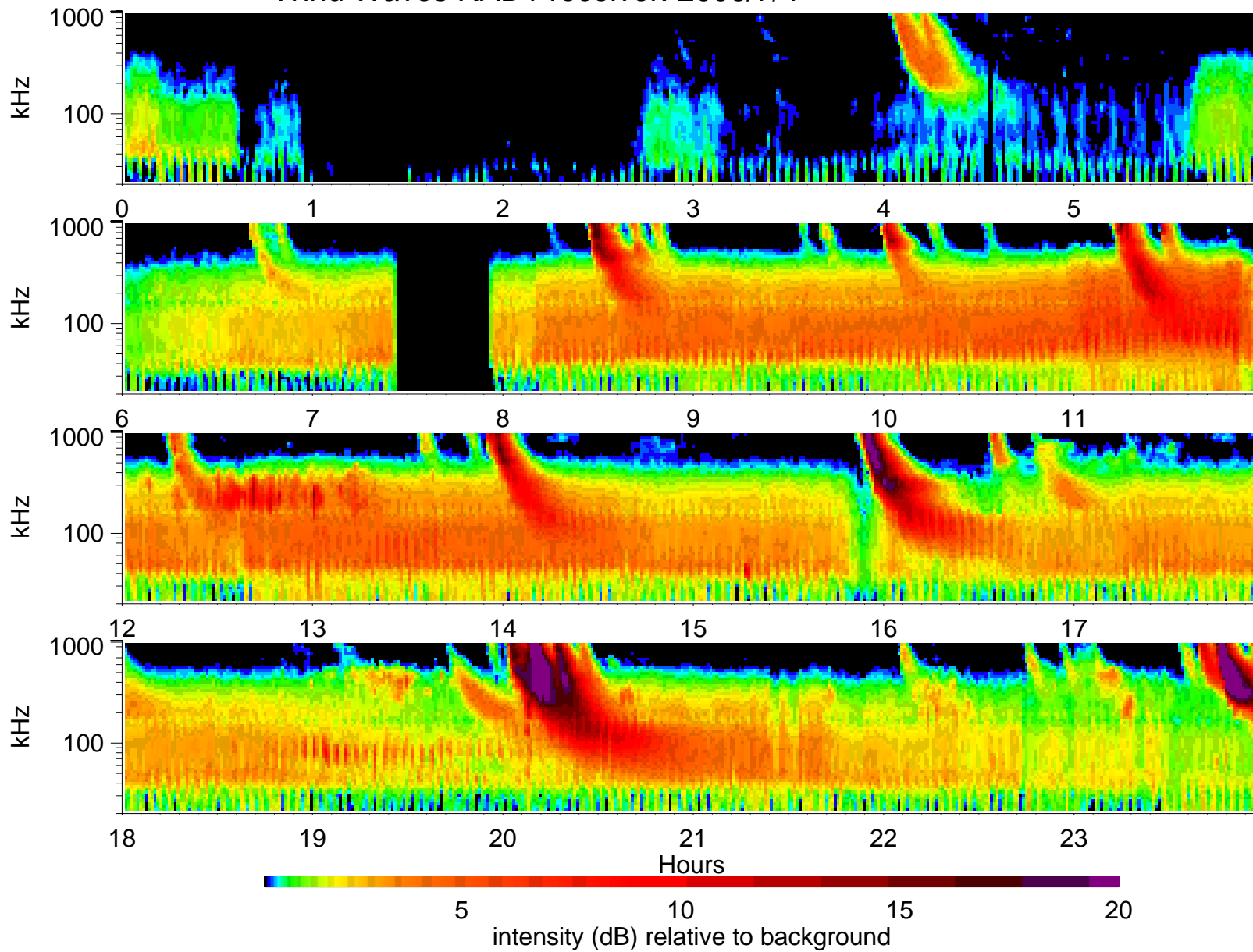
Wind Waves RAD1 receiver: 2006/7/4
