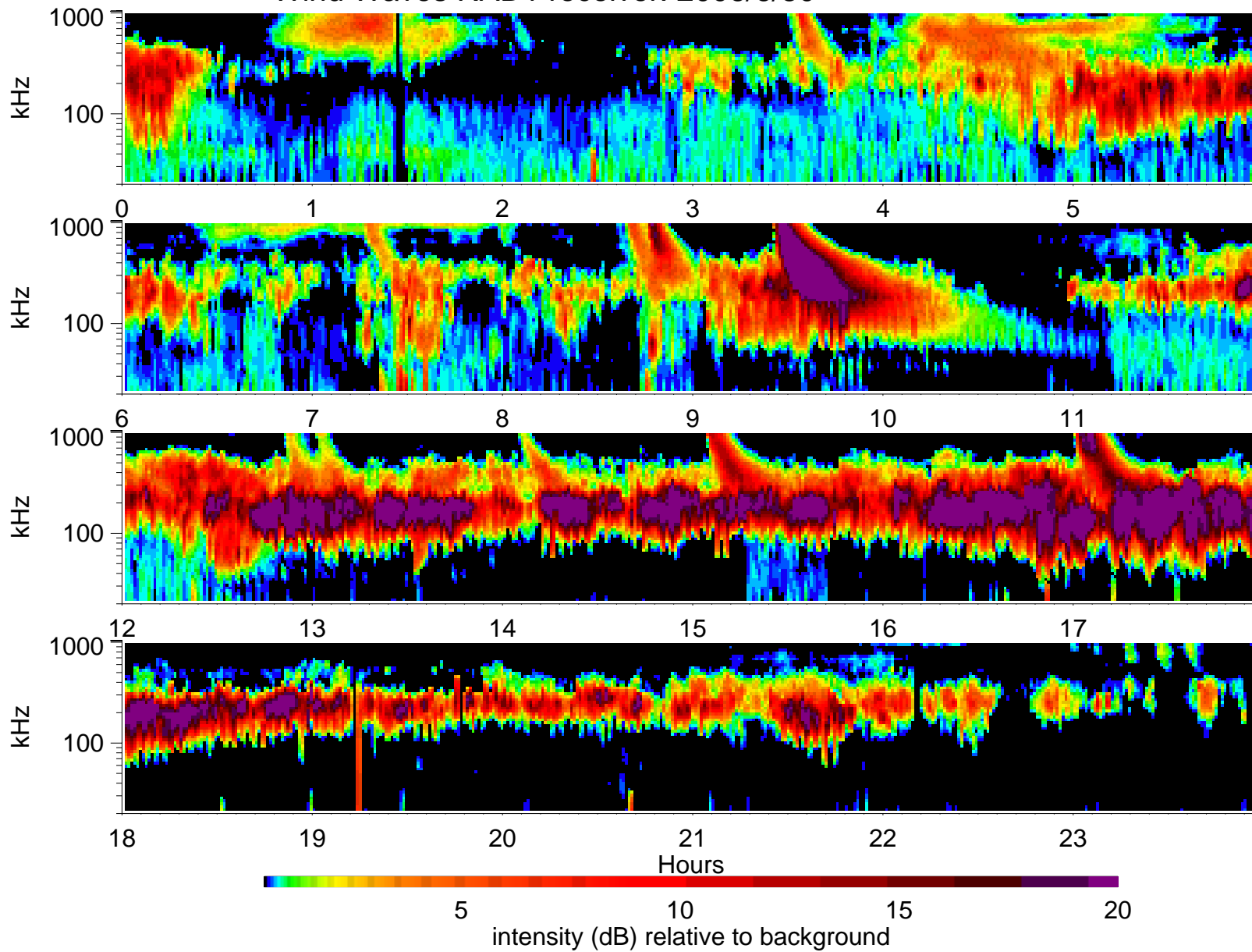
Wind Waves RAD1 receiver: 2006/6/30
