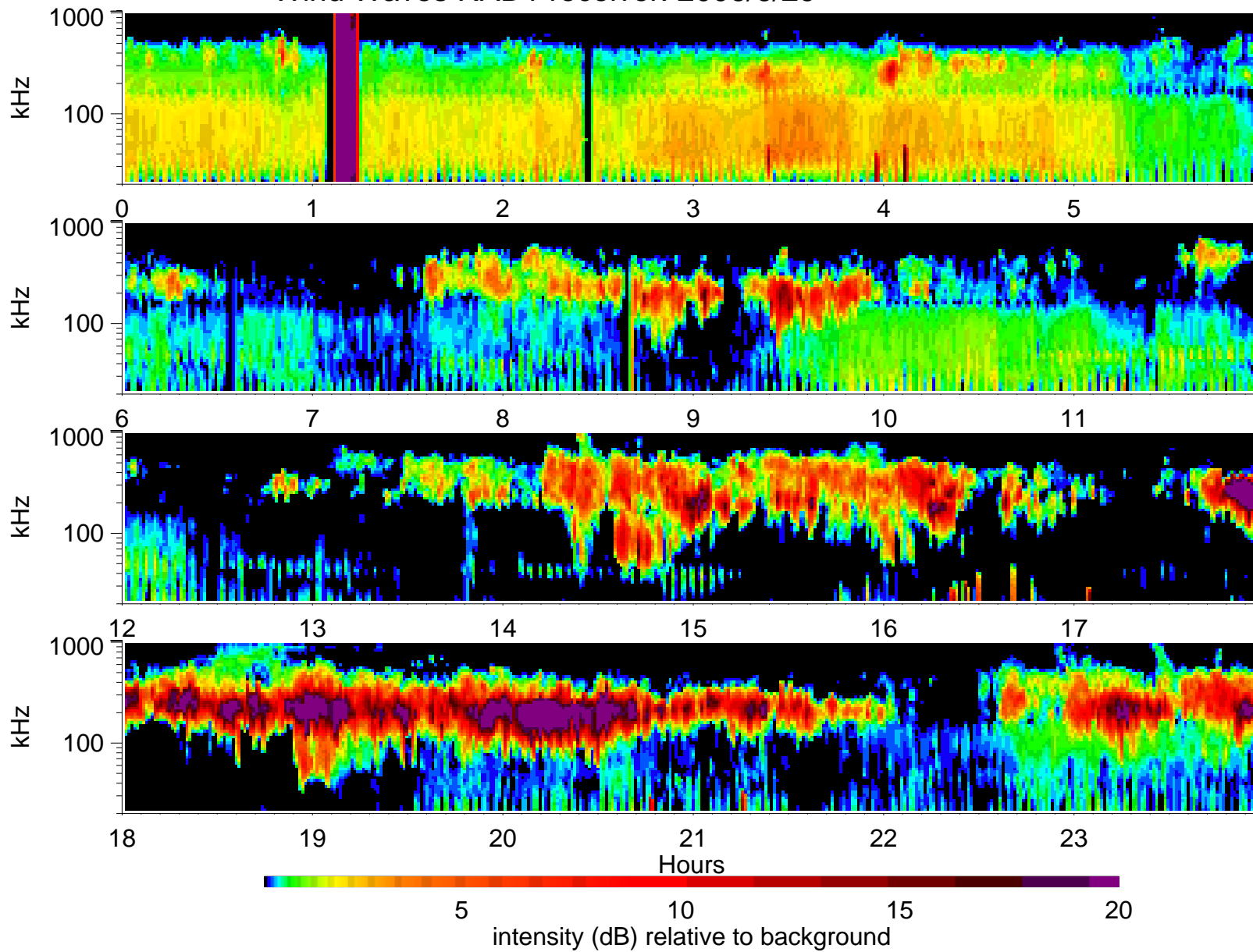
Wind Waves RAD1 receiver: 2006/6/29
