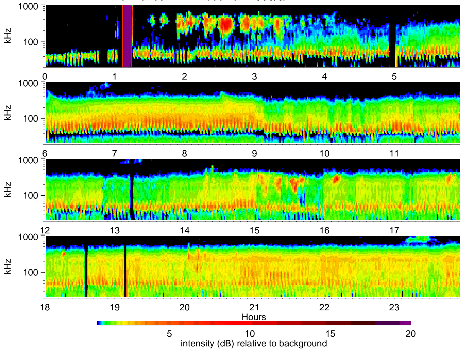
Wind Waves RAD1 receiver: 2006/6/27
