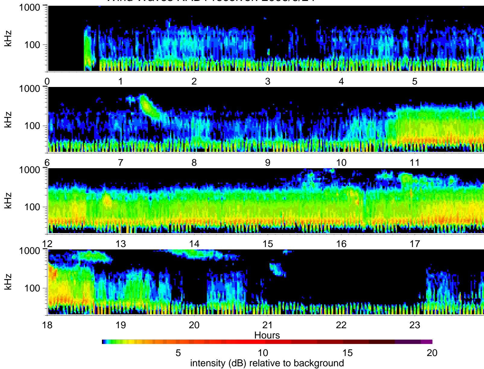
Wind Waves RAD1 receiver: 2006/6/24
