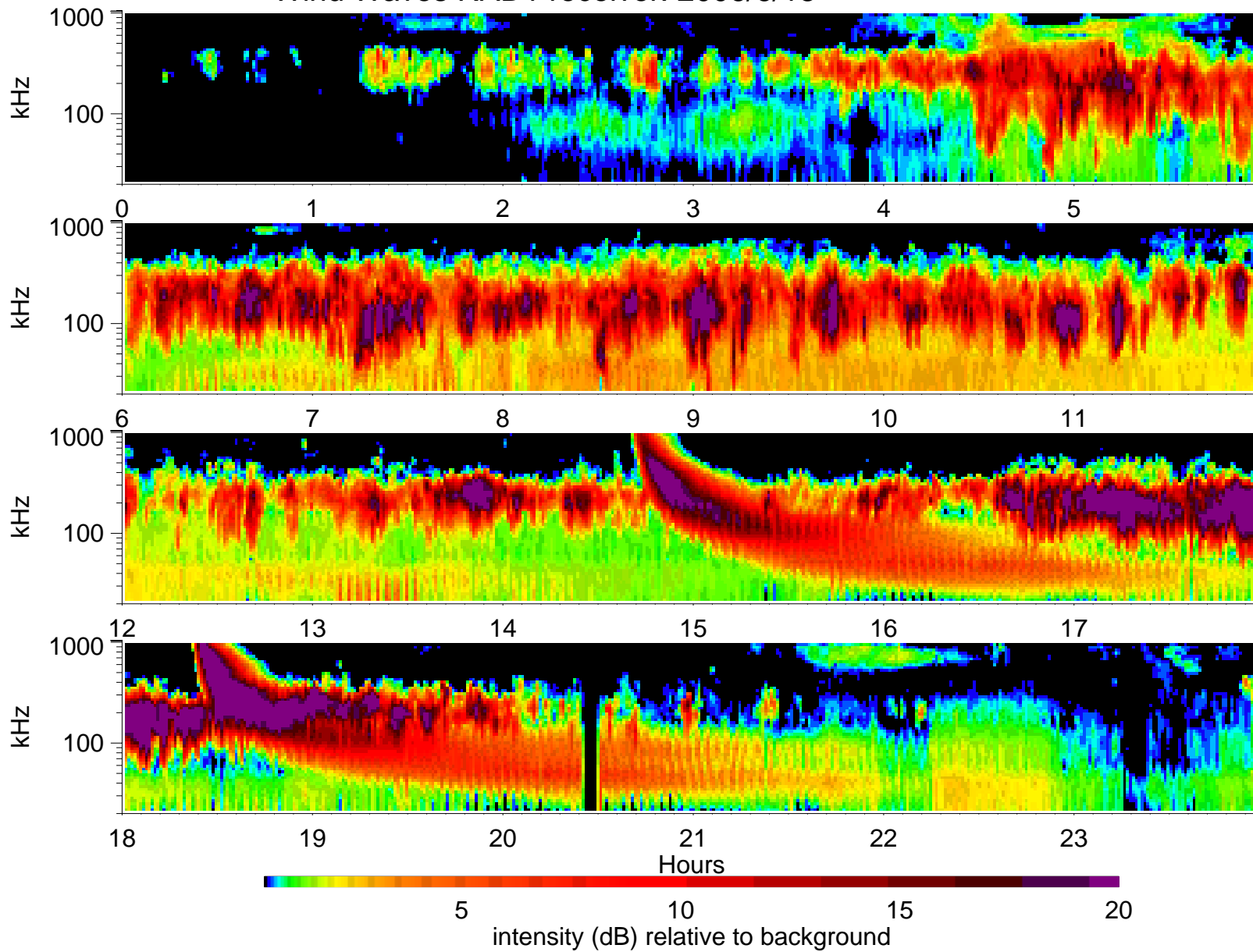
Wind Waves RAD1 receiver: 2006/6/18
