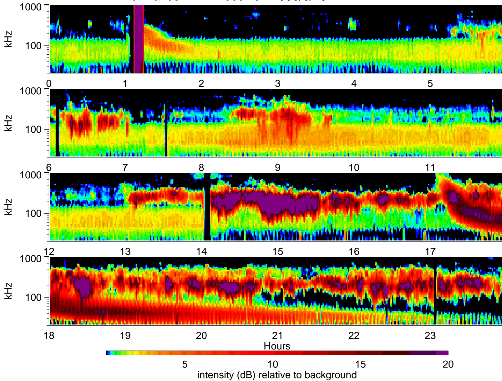
Wind Waves RAD1 receiver: 2006/6/15
