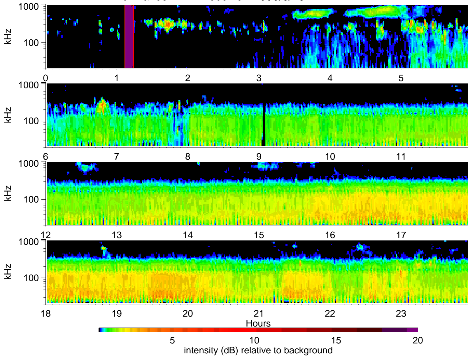
Wind Waves RAD1 receiver: 2006/6/13
