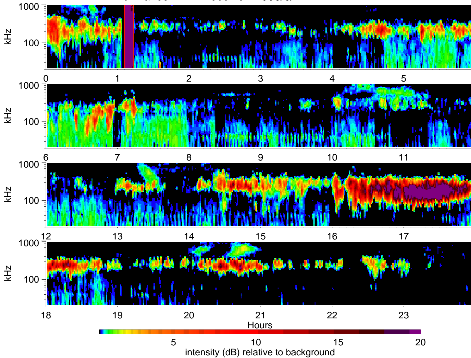
Wind Waves RAD1 receiver: 2006/6/11
