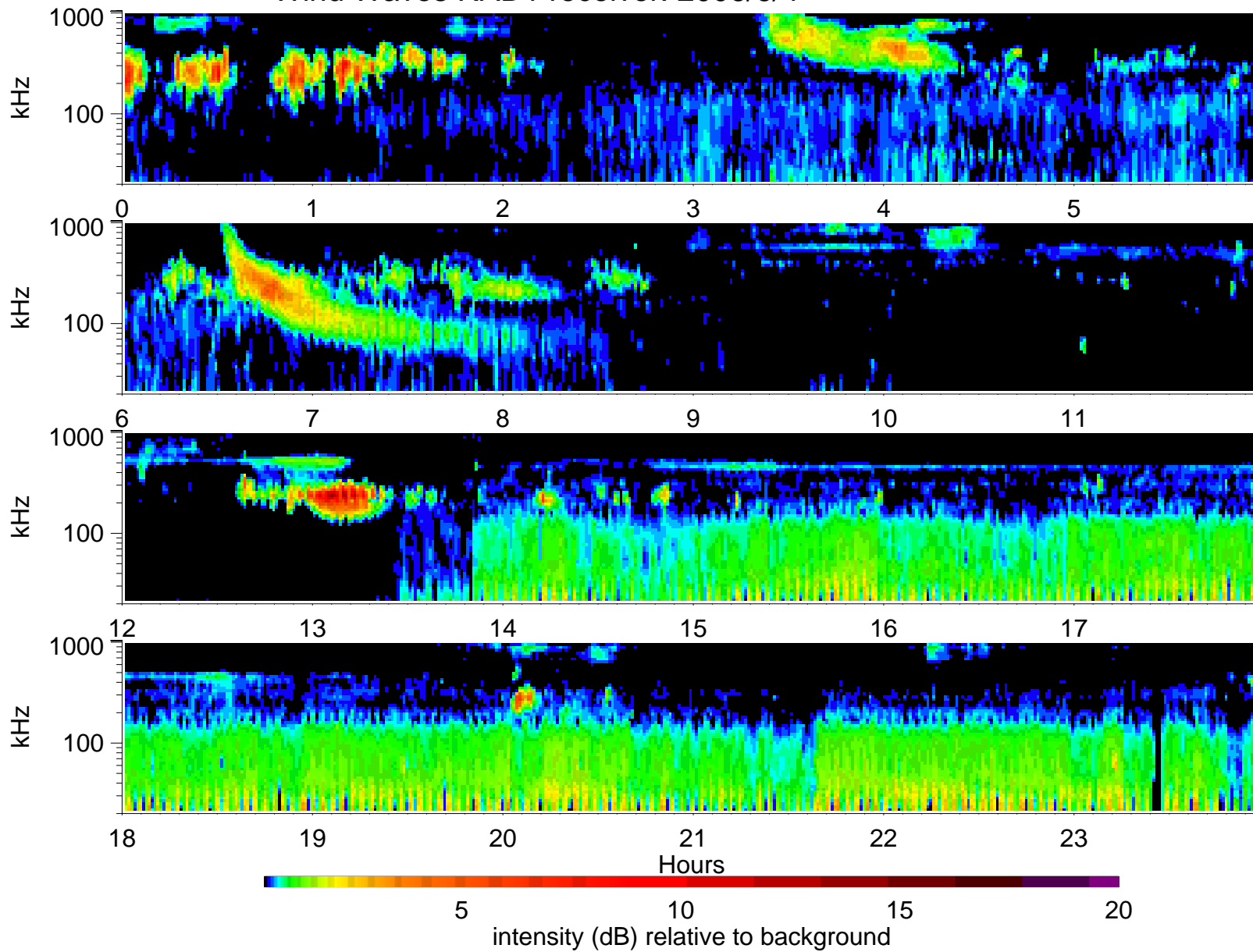
Wind Waves RAD1 receiver: 2006/6/4
