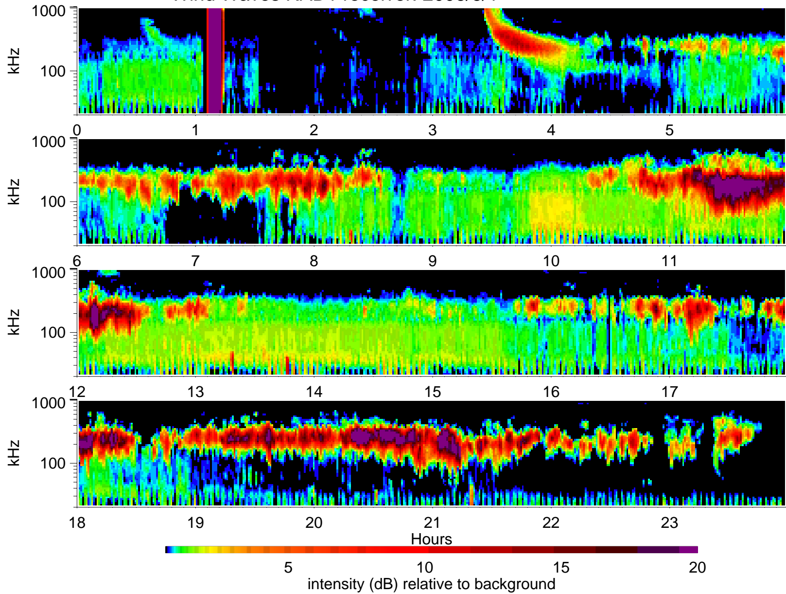
Wind Waves RAD1 receiver: 2006/6/1
