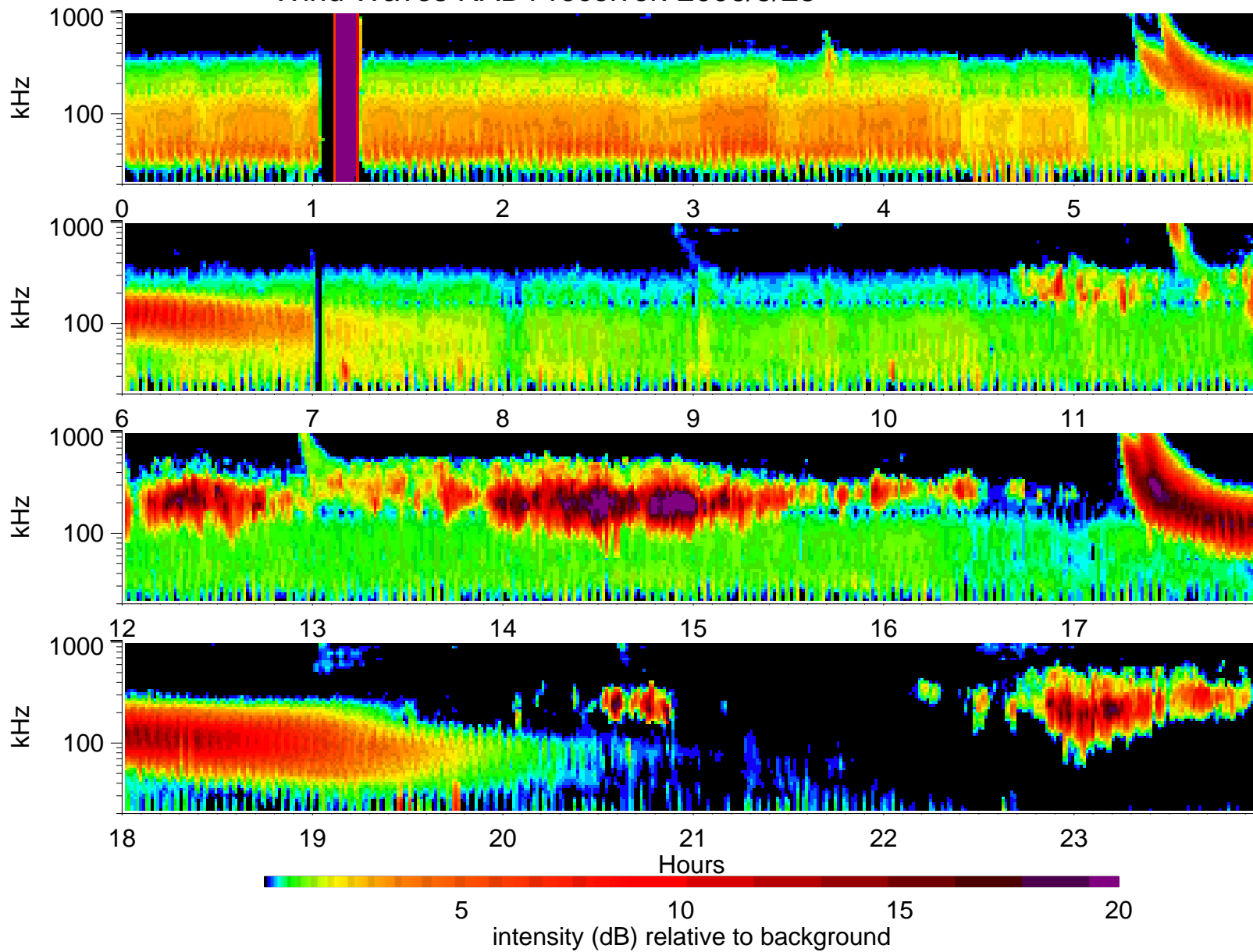
Wind Waves RAD1 receiver: 2006/5/28
