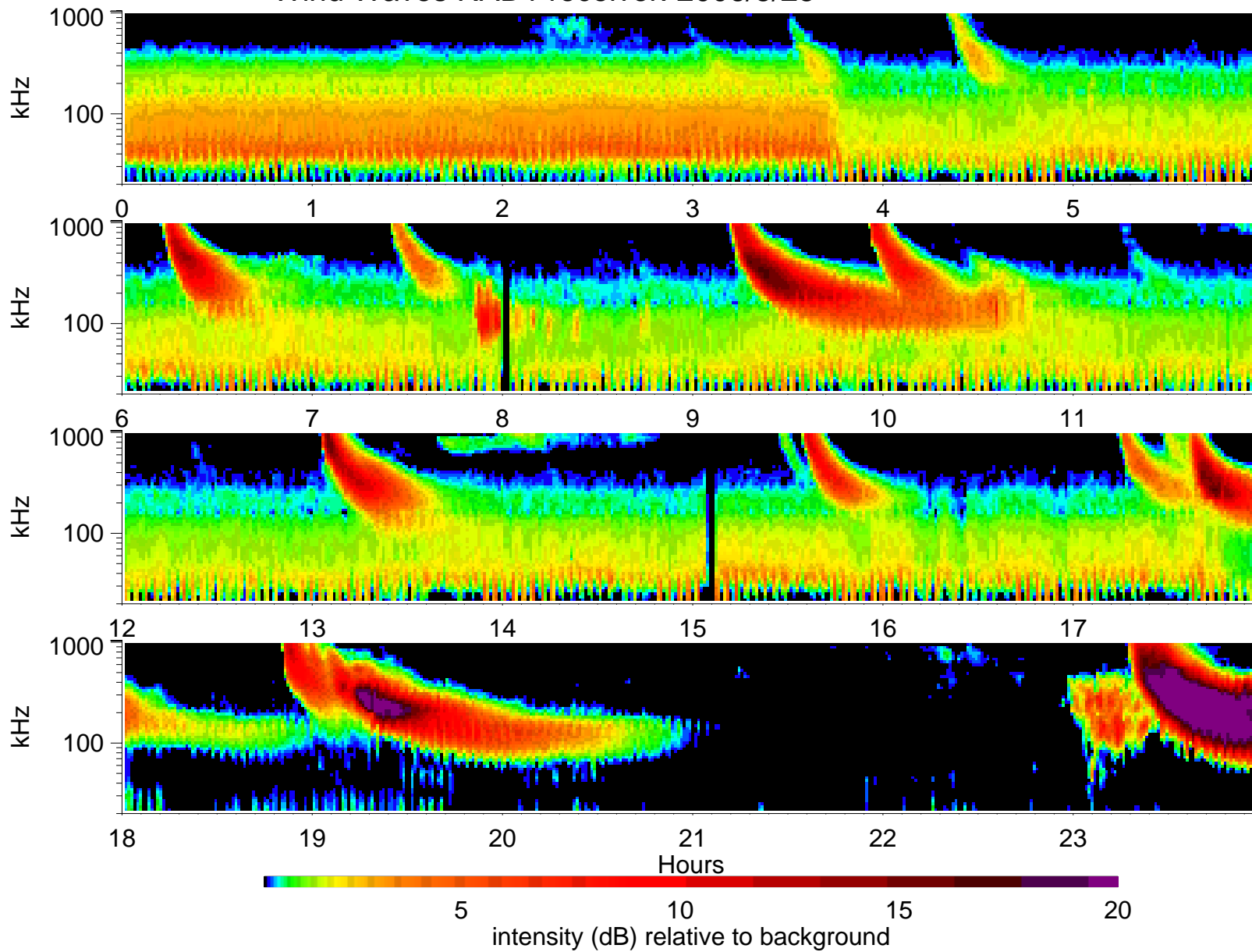
Wind Waves RAD1 receiver: 2006/5/25
