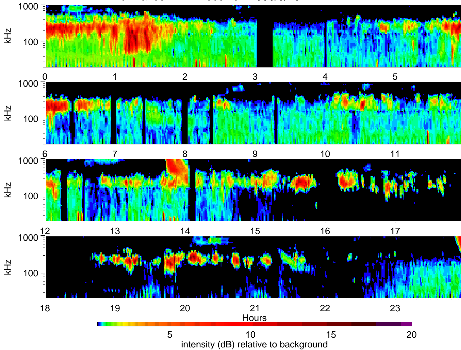
Wind Waves RAD1 receiver: 2006/5/23
