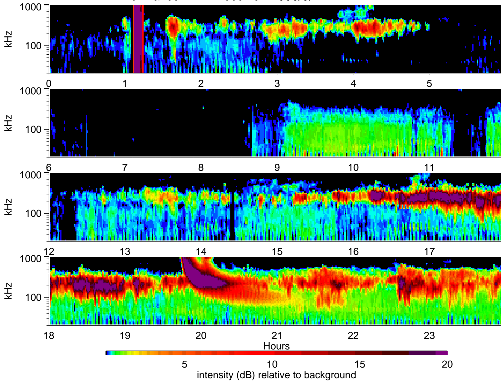
Wind Waves RAD1 receiver: 2006/5/22
