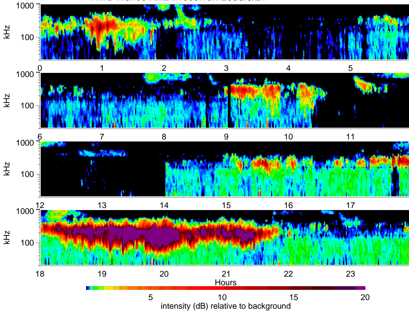
Wind Waves RAD1 receiver: 2006/5/21
