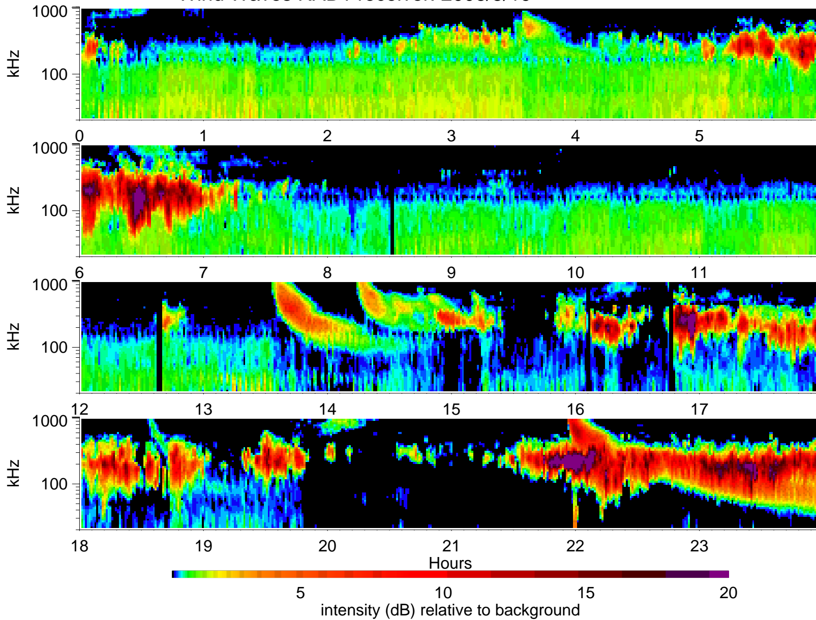
Wind Waves RAD1 receiver: 2006/5/19
