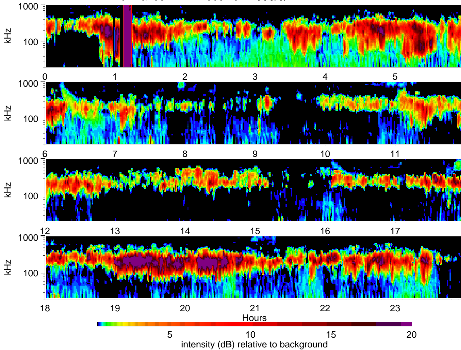
Wind Waves RAD1 receiver: 2006/5/14
