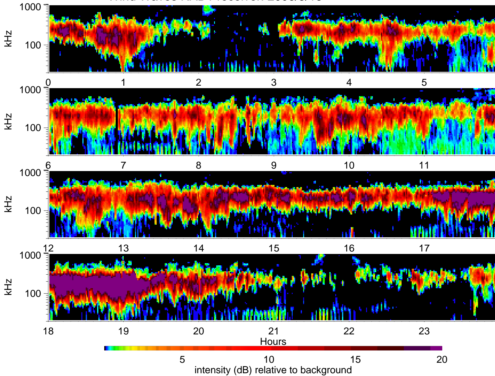
Wind Waves RAD1 receiver: 2006/5/13
