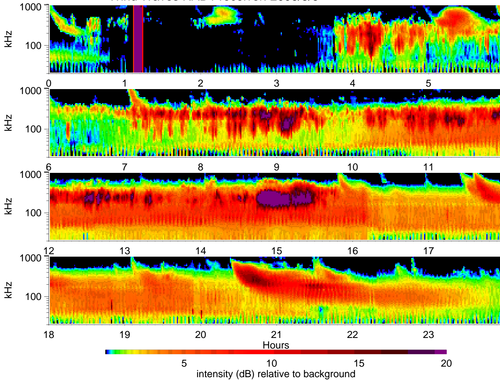
Wind Waves RAD1 receiver: 2006/5/6
