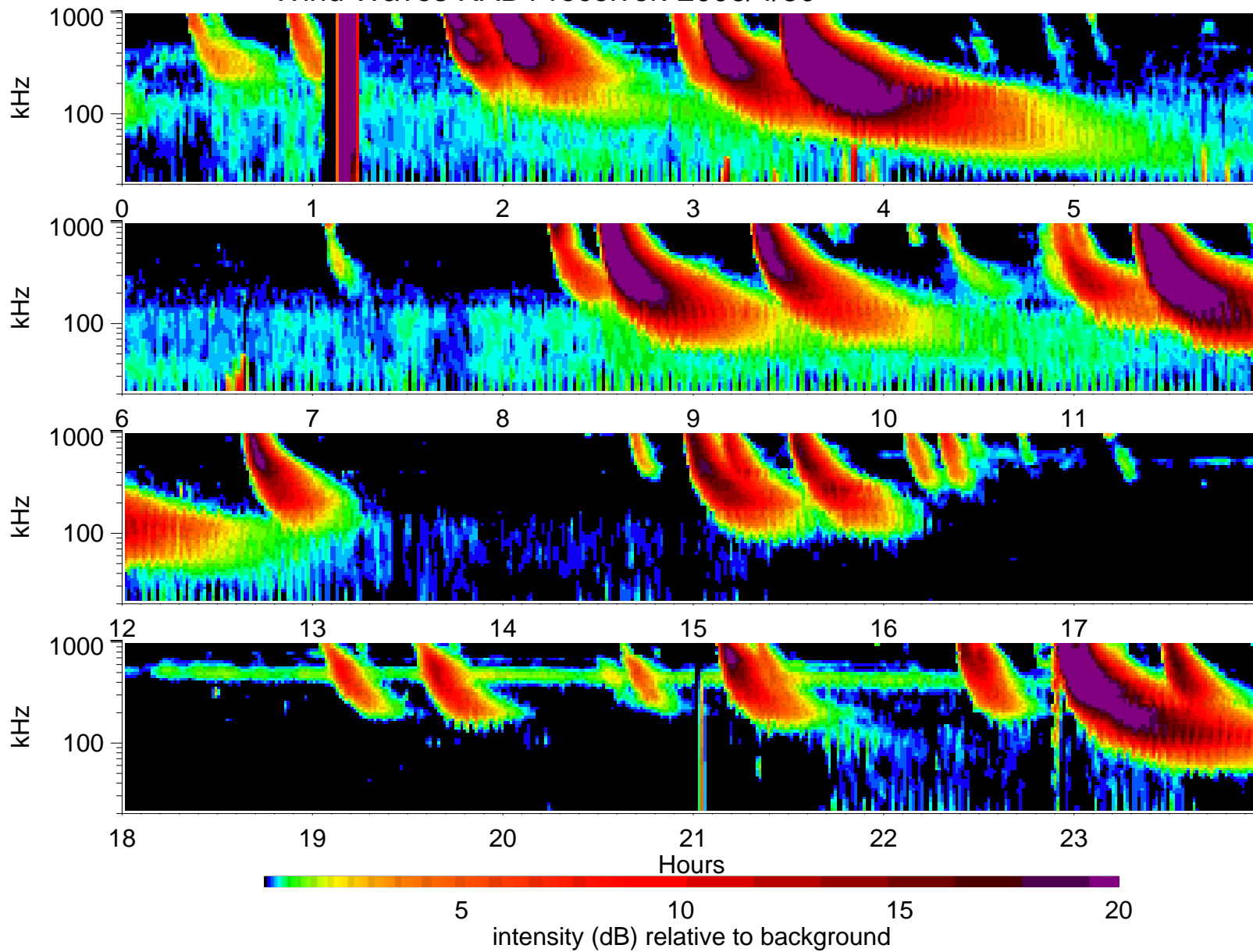
Wind Waves RAD1 receiver: 2006/4/30
