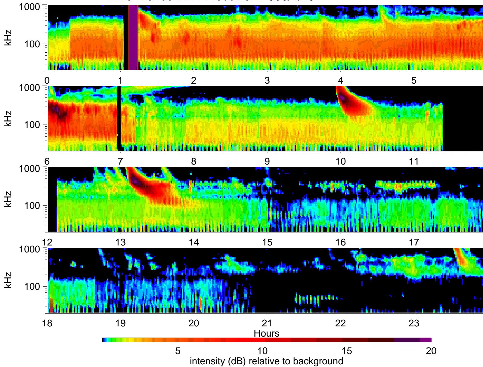
Wind Waves RAD1 receiver: 2006/4/28
