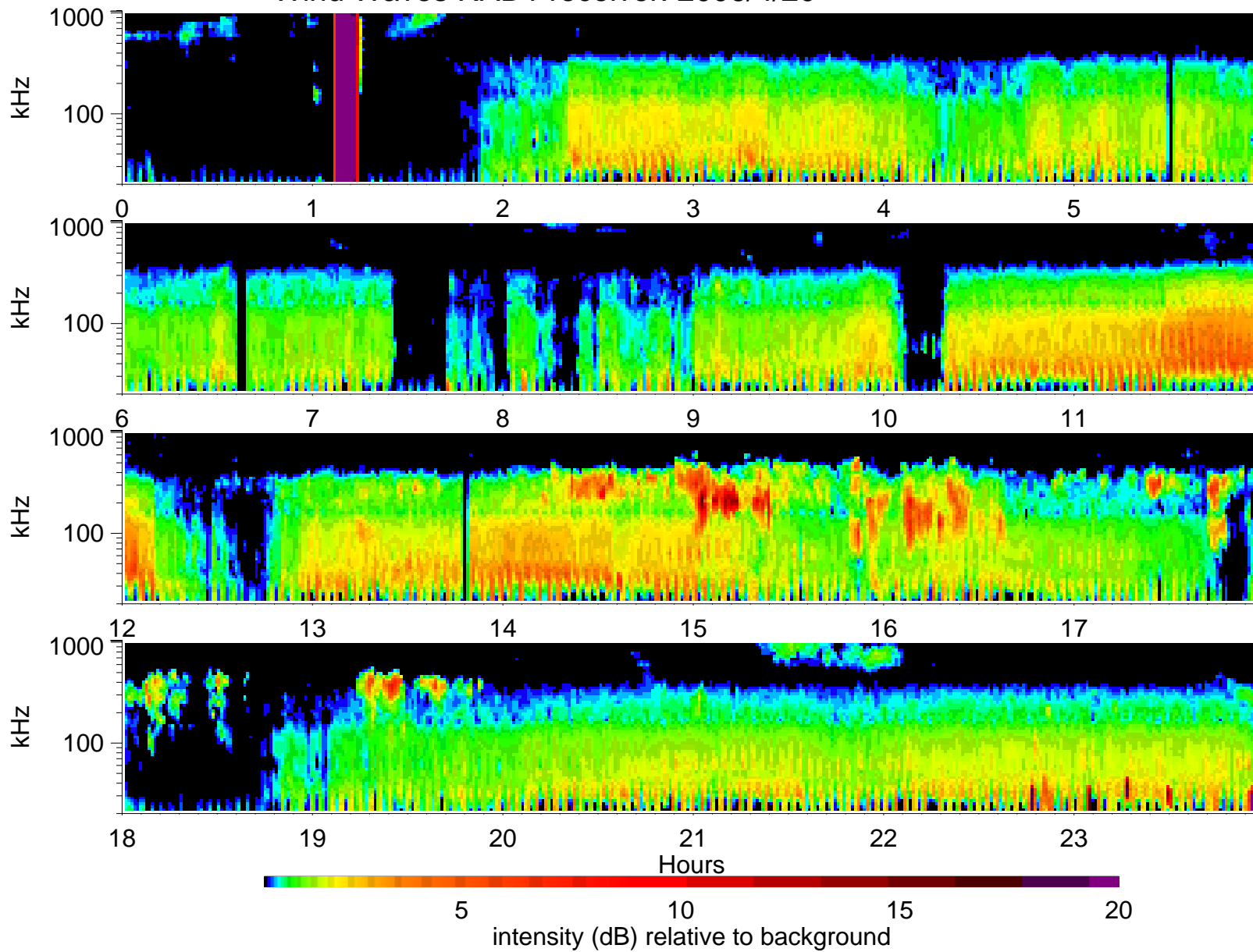
Wind Waves RAD1 receiver: 2006/4/20
