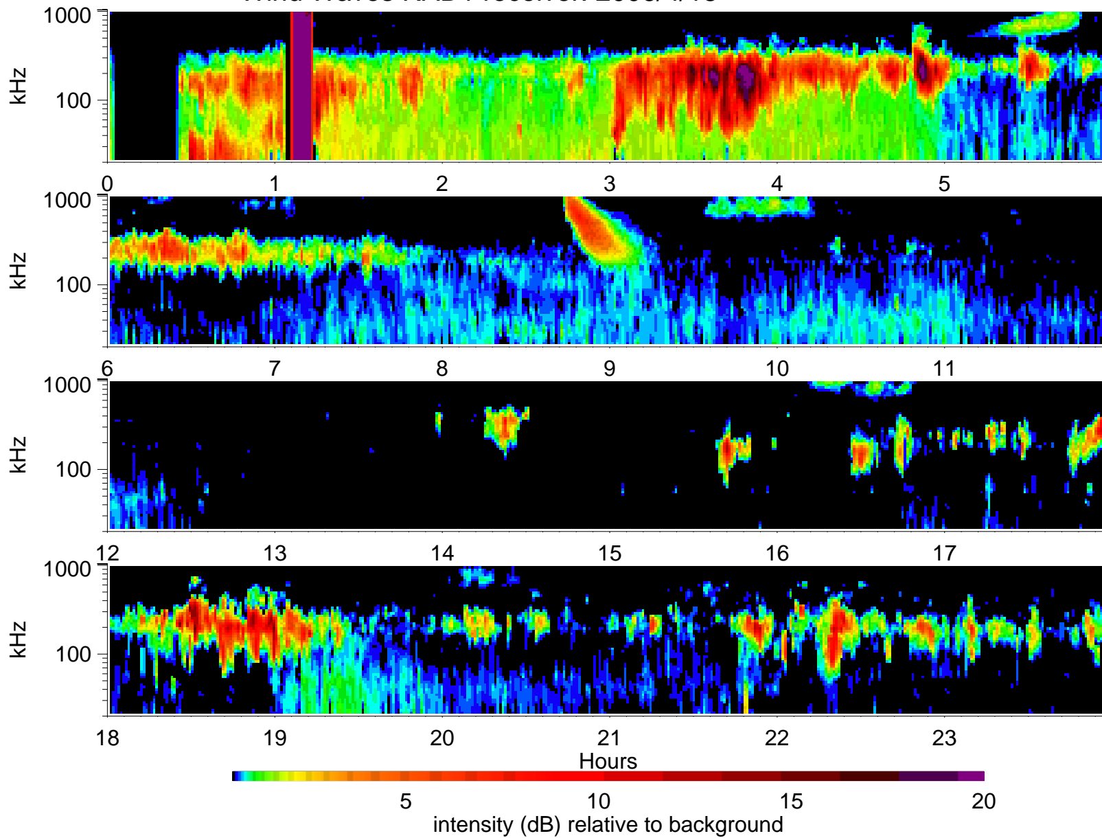
Wind Waves RAD1 receiver: 2006/4/18
