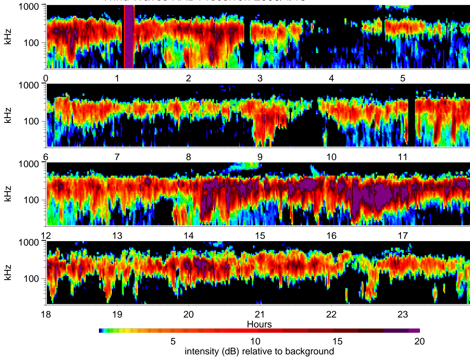
Wind Waves RAD1 receiver: 2006/4/16
