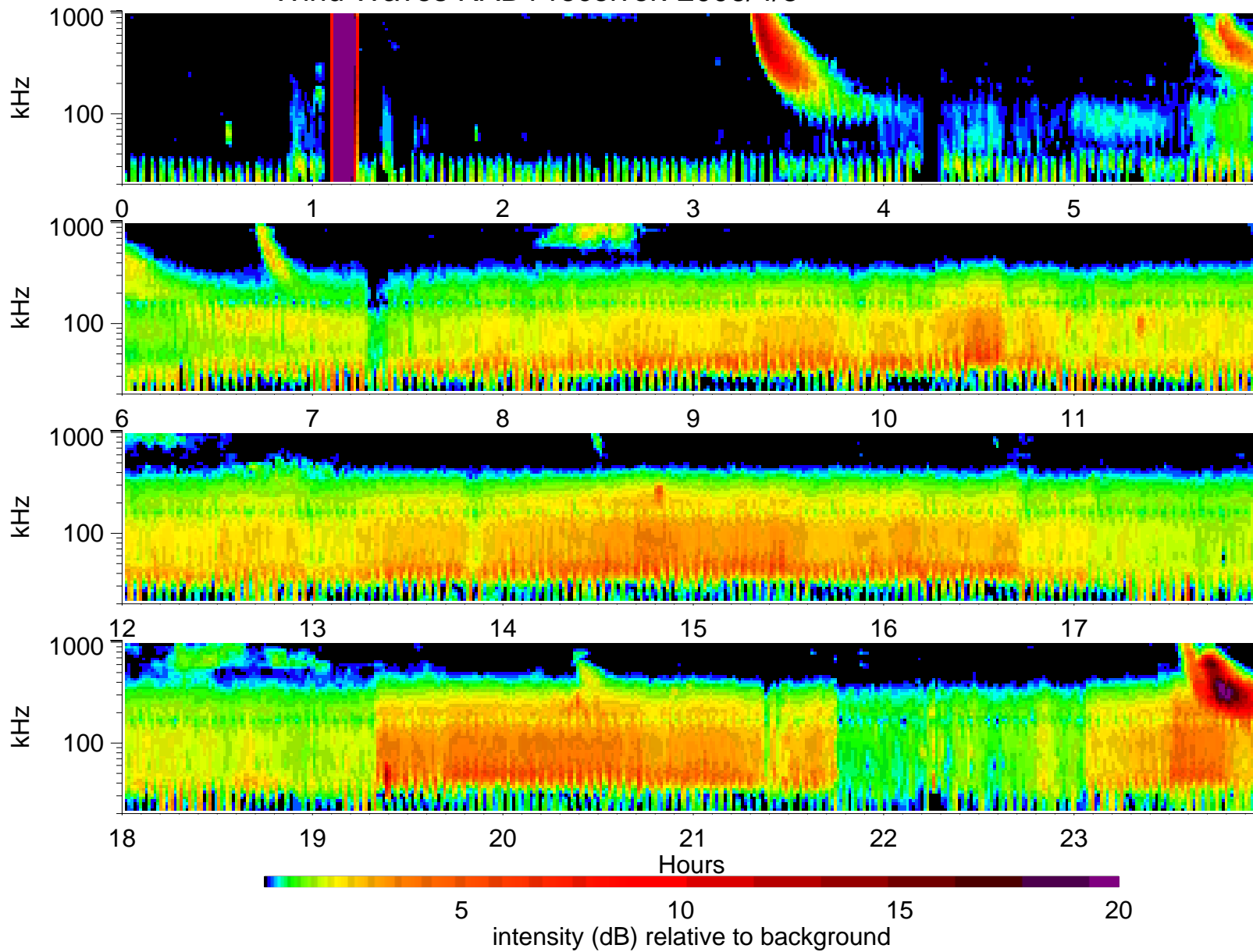
Wind Waves RAD1 receiver: 2006/4/8
