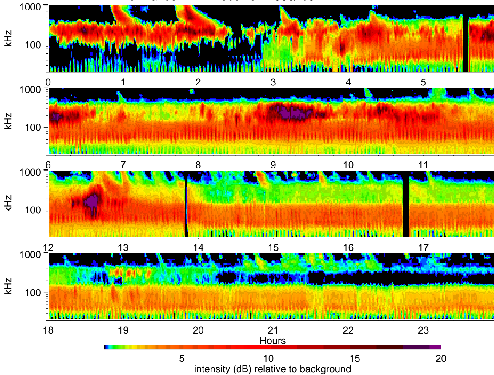
Wind Waves RAD1 receiver: 2006/4/5
