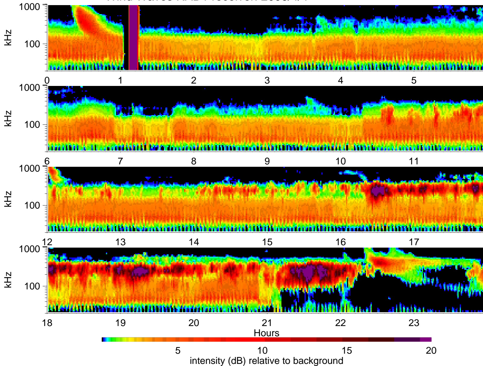
Wind Waves RAD1 receiver: 2006/4/4
