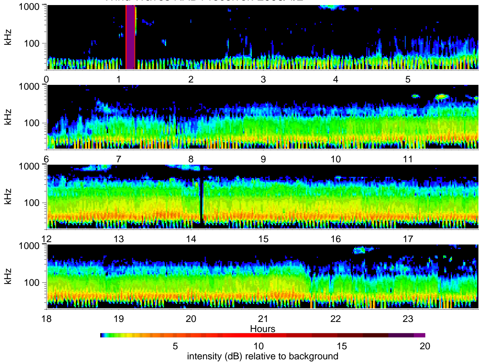
Wind Waves RAD1 receiver: 2006/4/2
