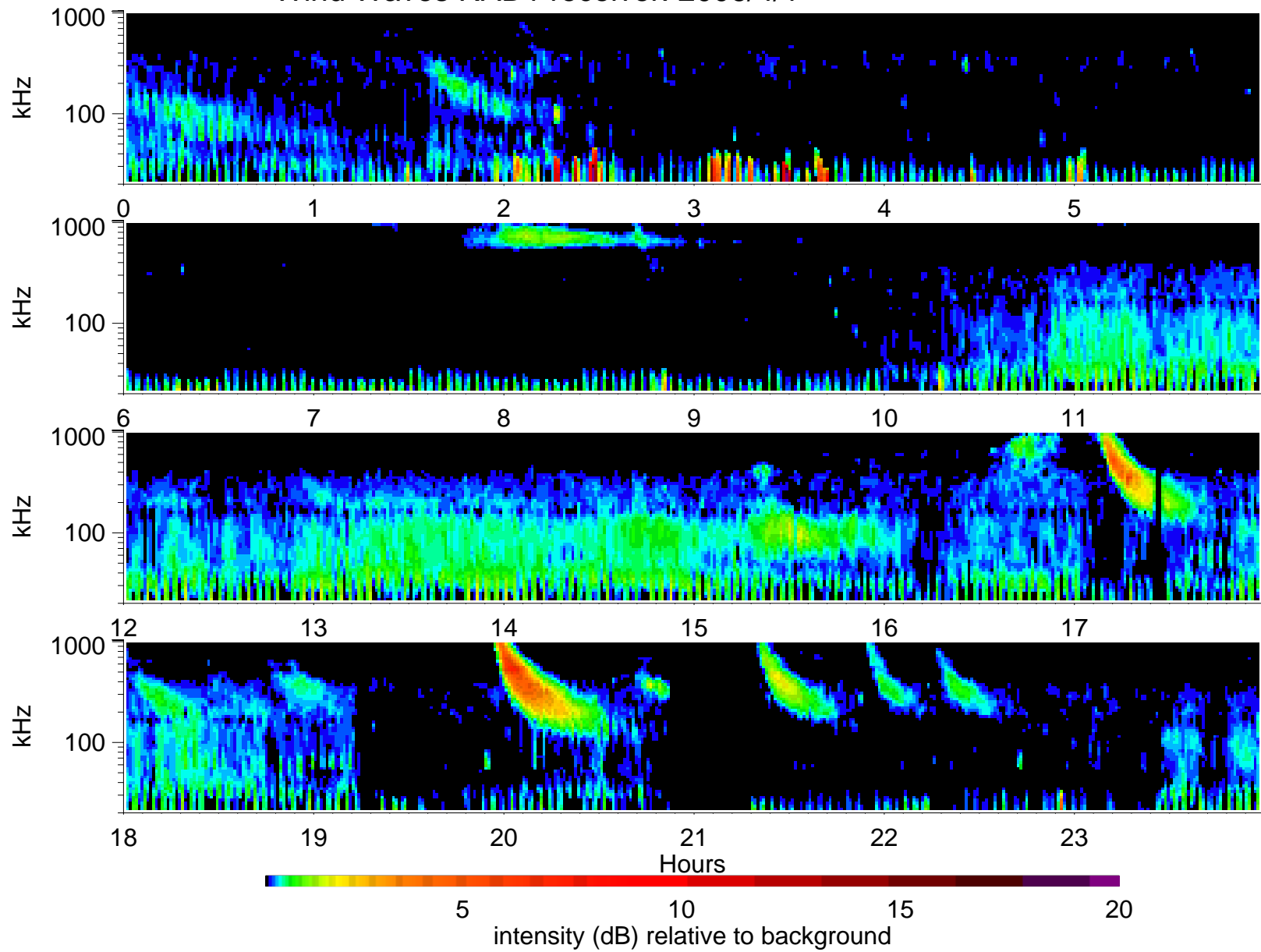
Wind Waves RAD1 receiver: 2006/4/1
