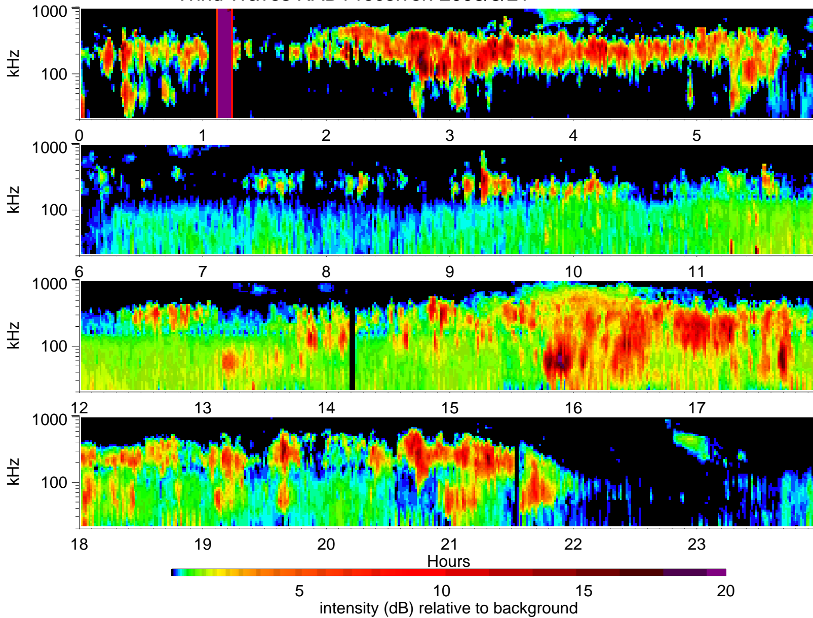
Wind Waves RAD1 receiver: 2006/3/21
