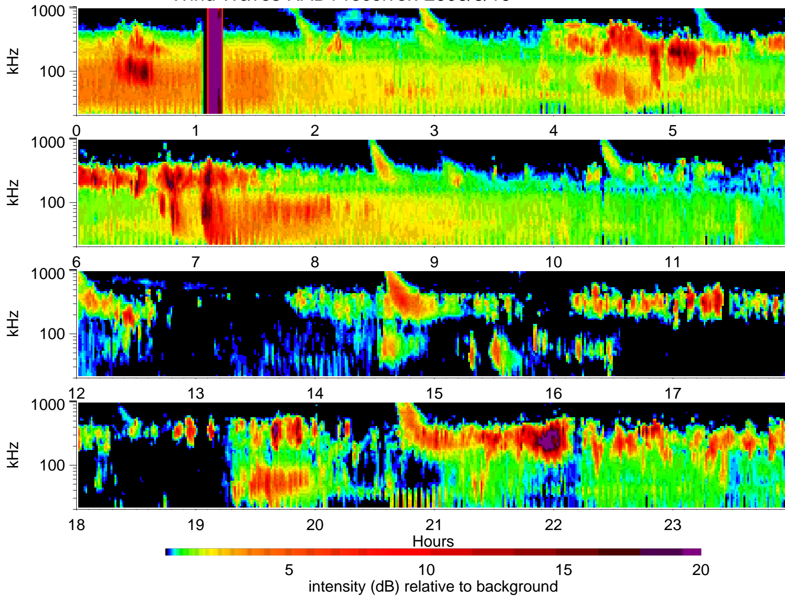
Wind Waves RAD1 receiver: 2006/3/19
