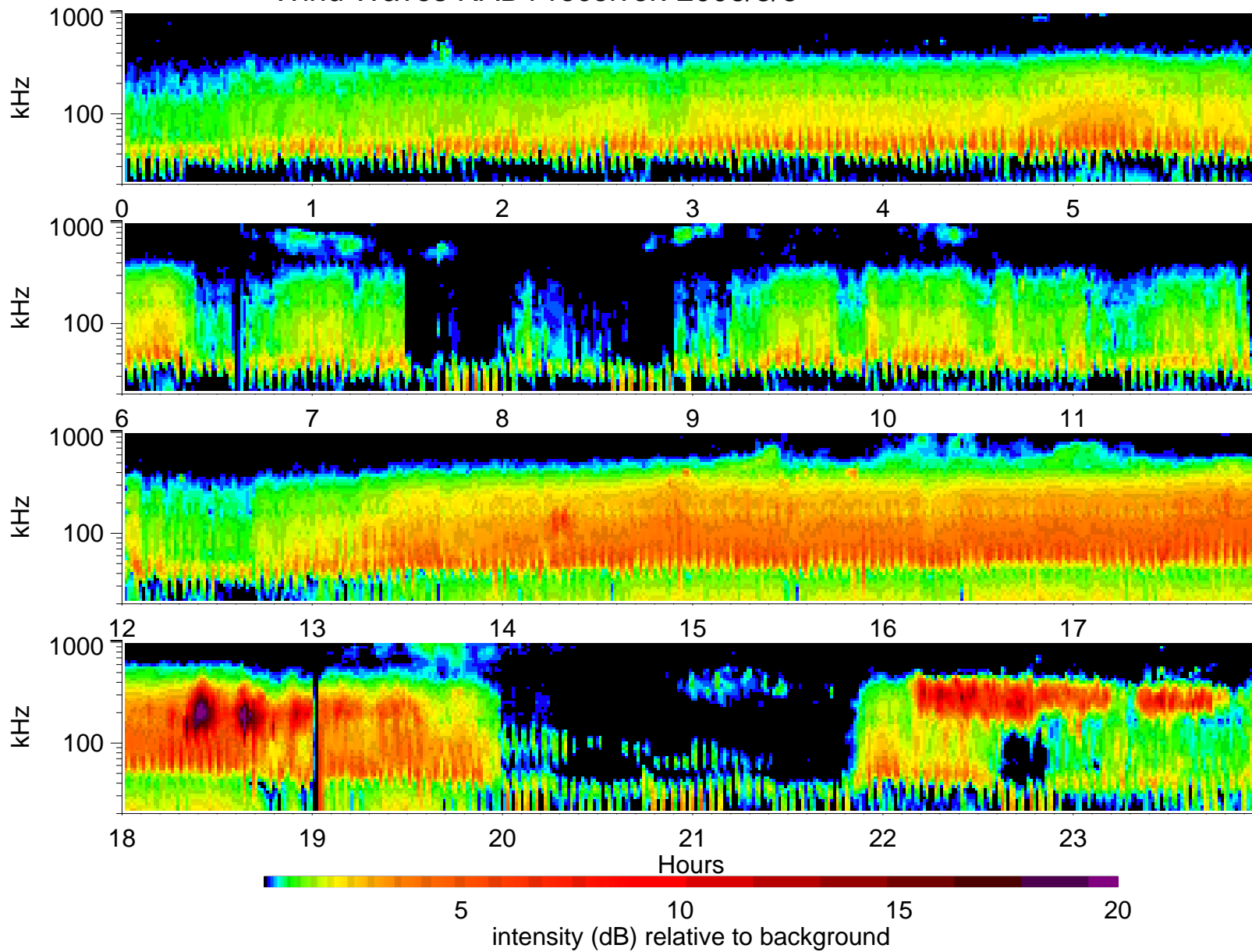
Wind Waves RAD1 receiver: 2006/3/6
