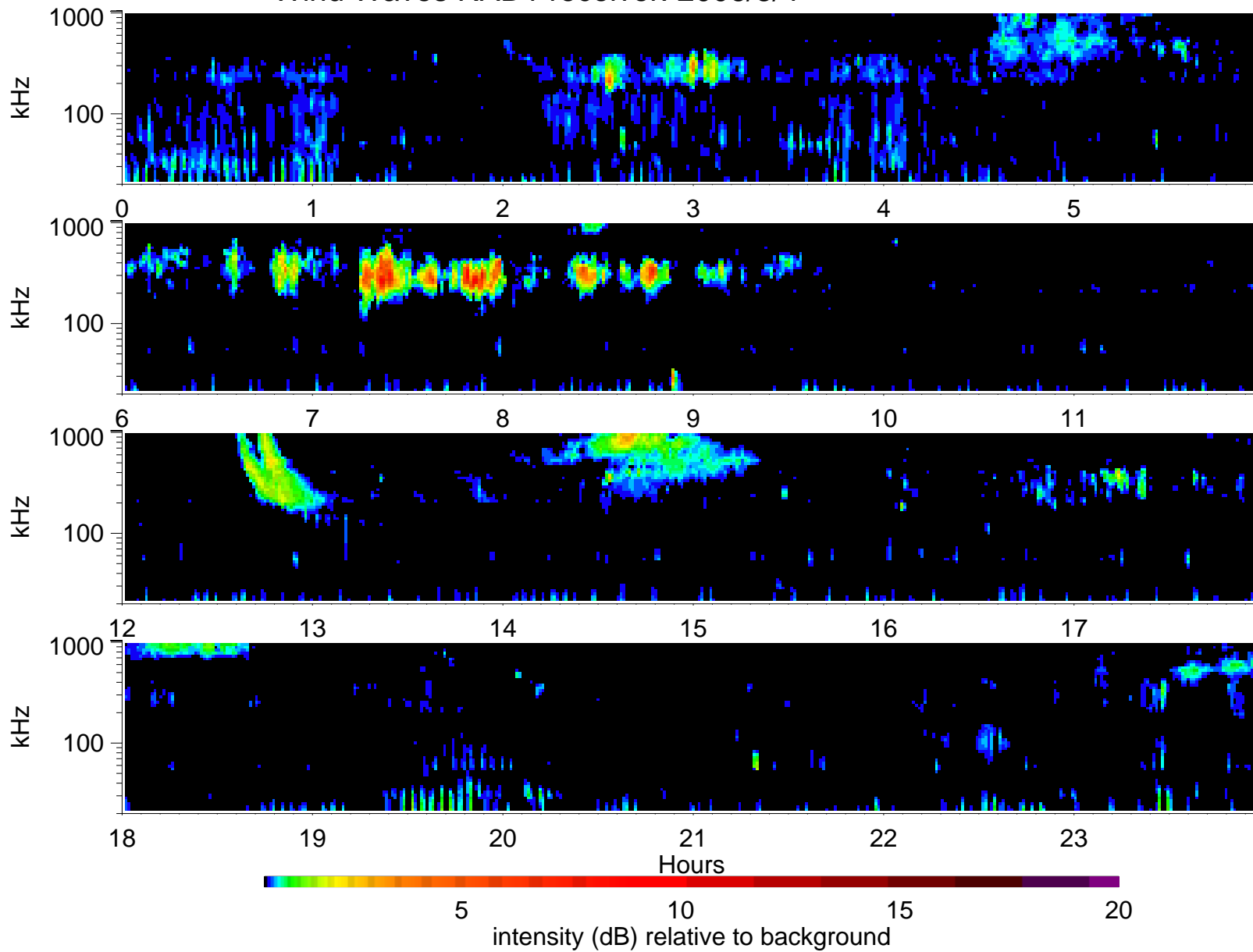
Wind Waves RAD1 receiver: 2006/3/4
