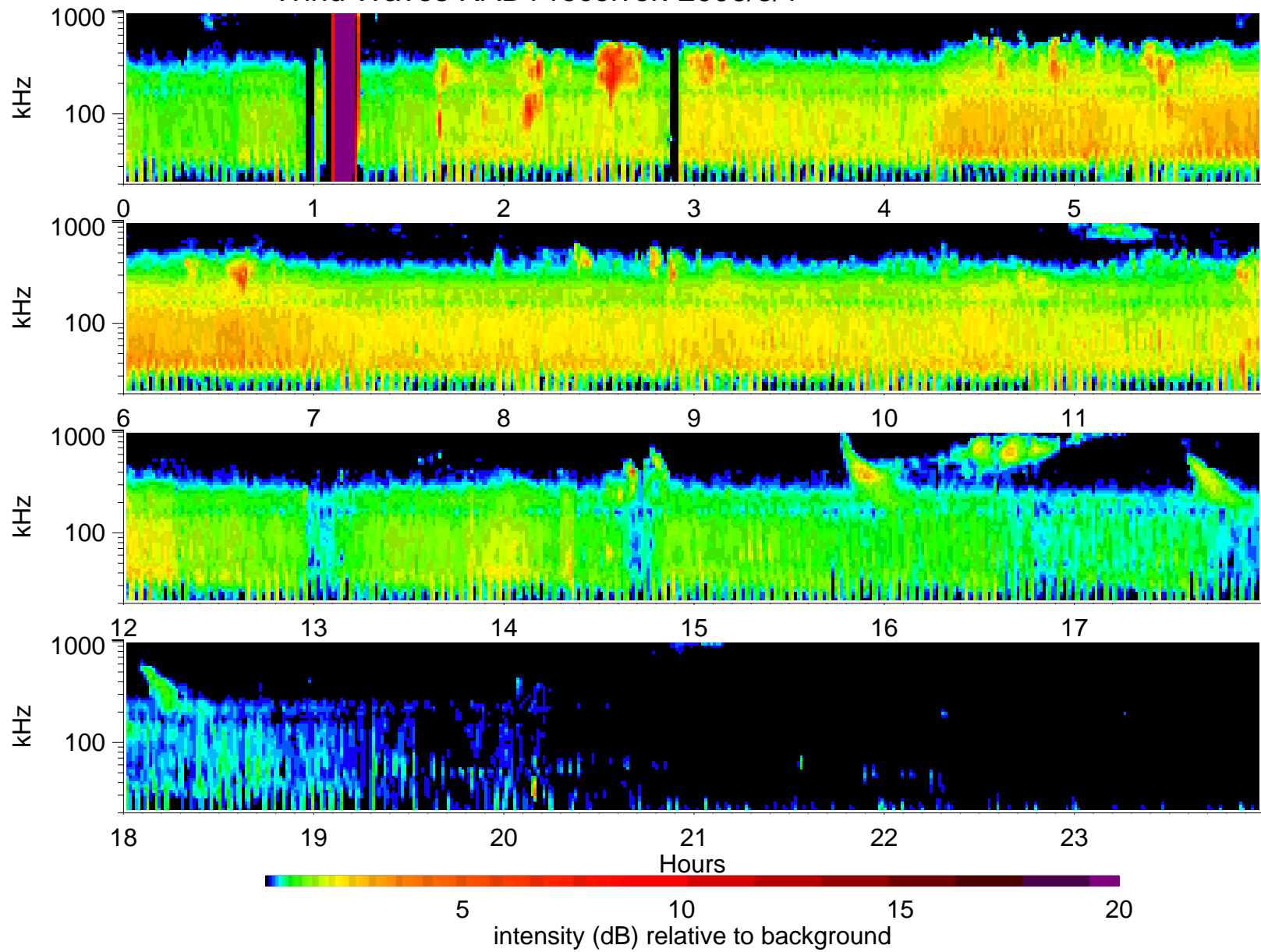
Wind Waves RAD1 receiver: 2006/3/1
