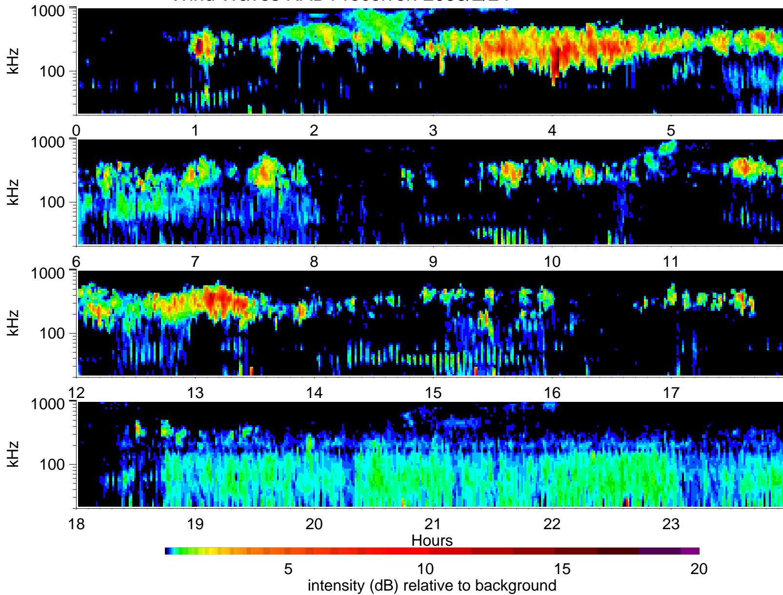
Wind Waves RAD1 receiver: 2006/2/24
