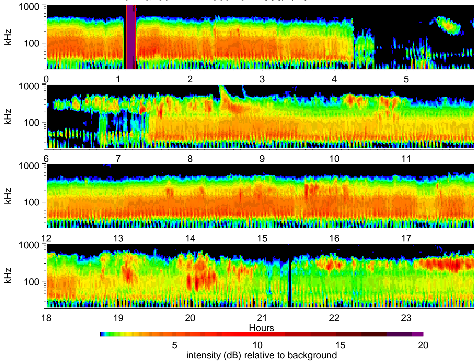
Wind Waves RAD1 receiver: 2006/2/19
