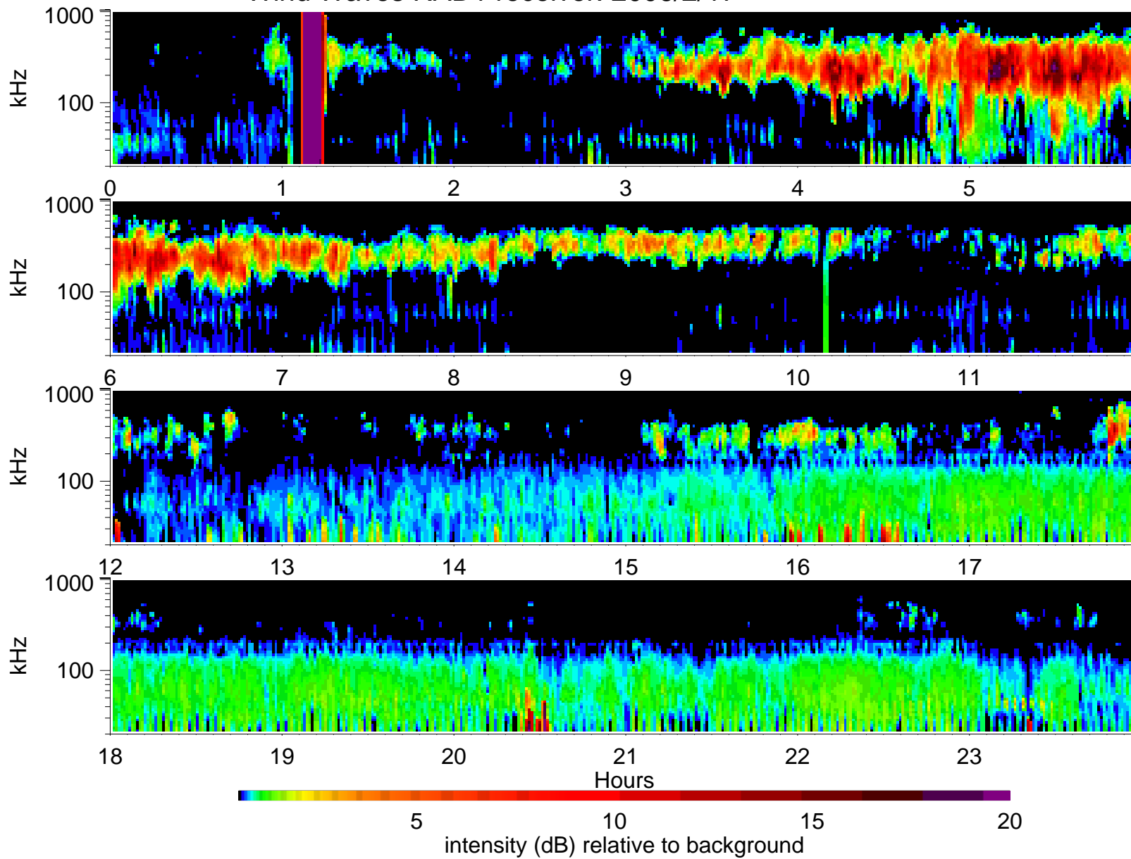
Wind Waves RAD1 receiver: 2006/2/17
