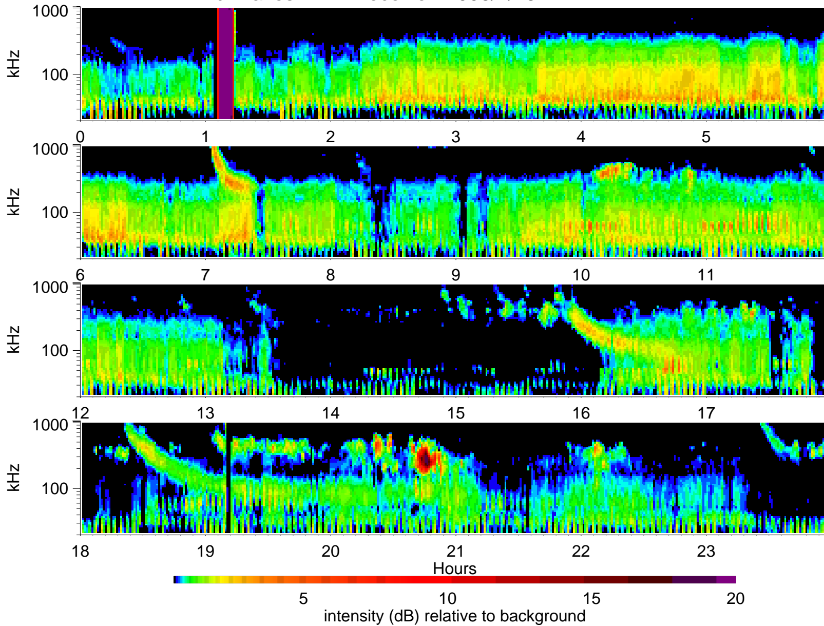
Wind Waves RAD1 receiver: 2006/2/15
