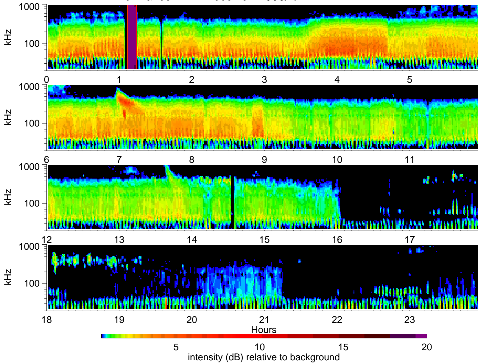
Wind Waves RAD1 receiver: 2006/2/11
