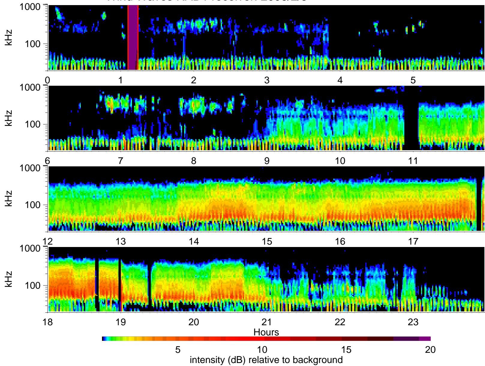
Wind Waves RAD1 receiver: 2006/2/5
