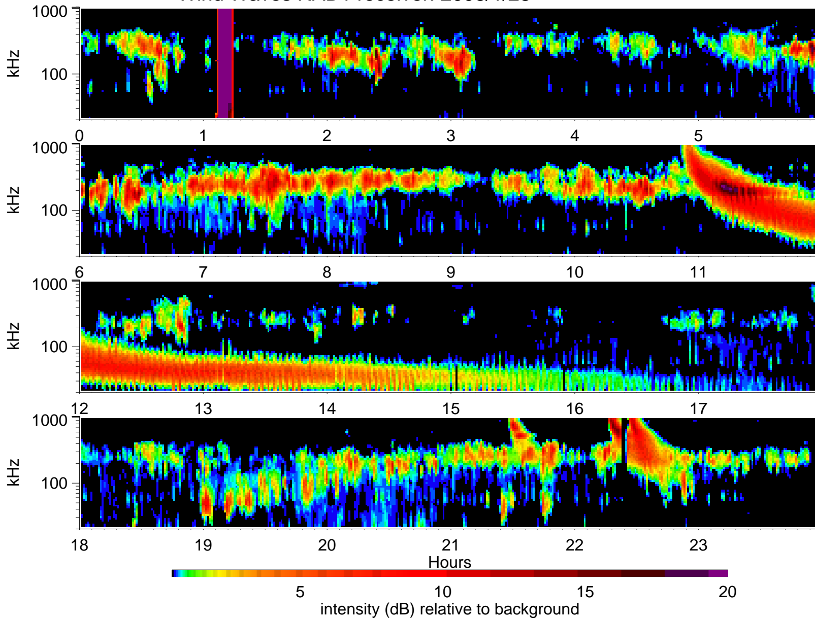
Wind Waves RAD1 receiver: 2006/1/28
