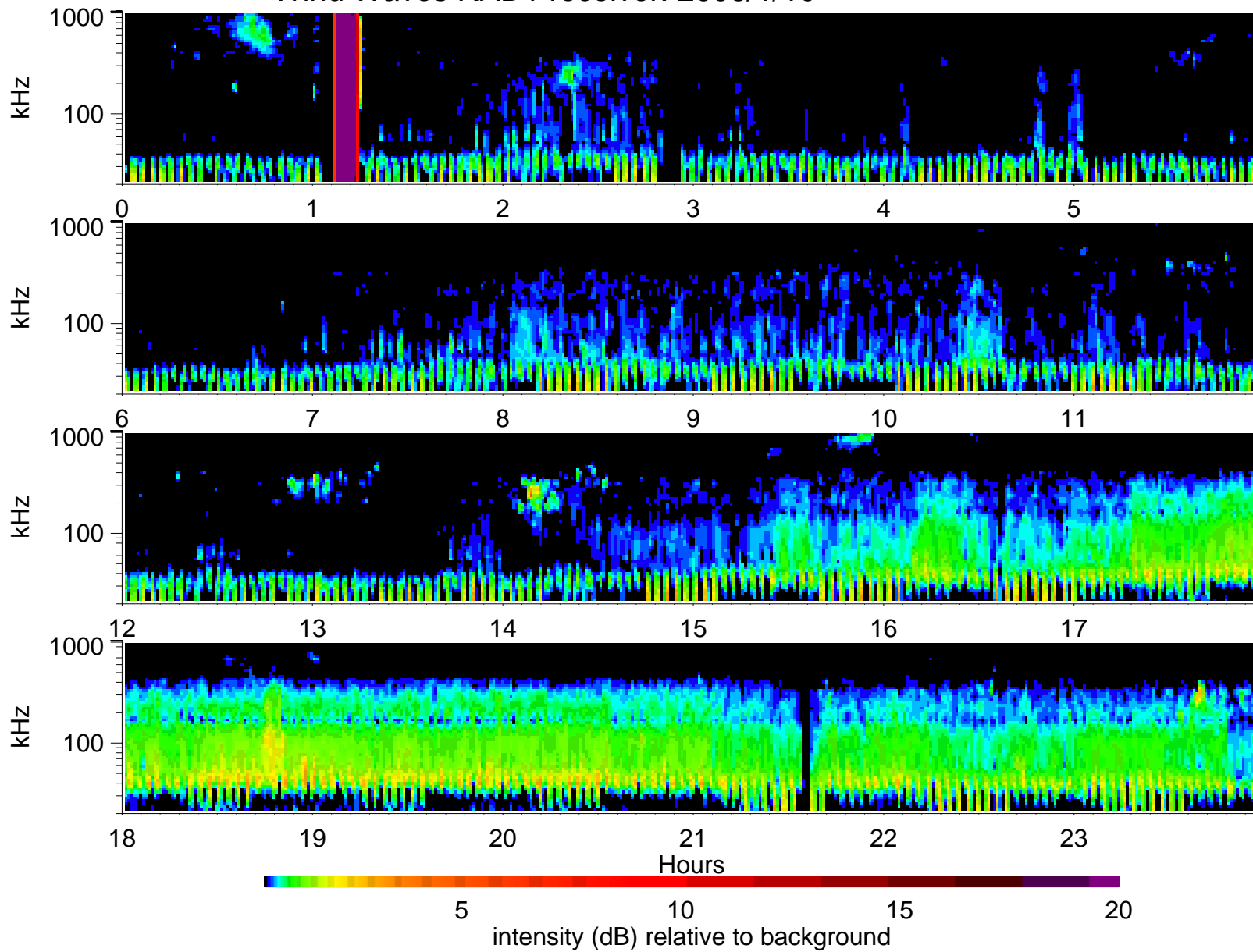
Wind Waves RAD1 receiver: 2006/1/10
