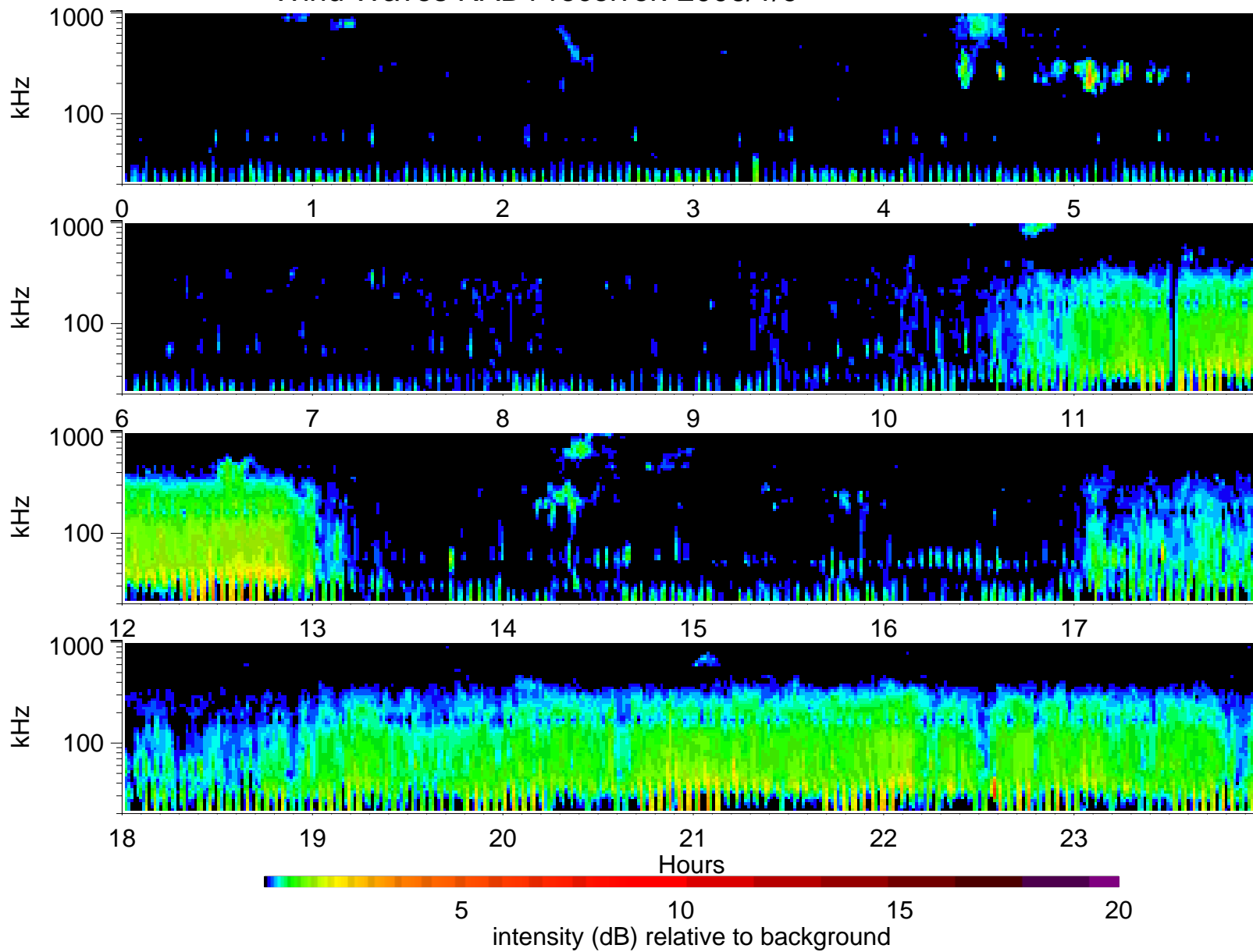
Wind Waves RAD1 receiver: 2006/1/9
