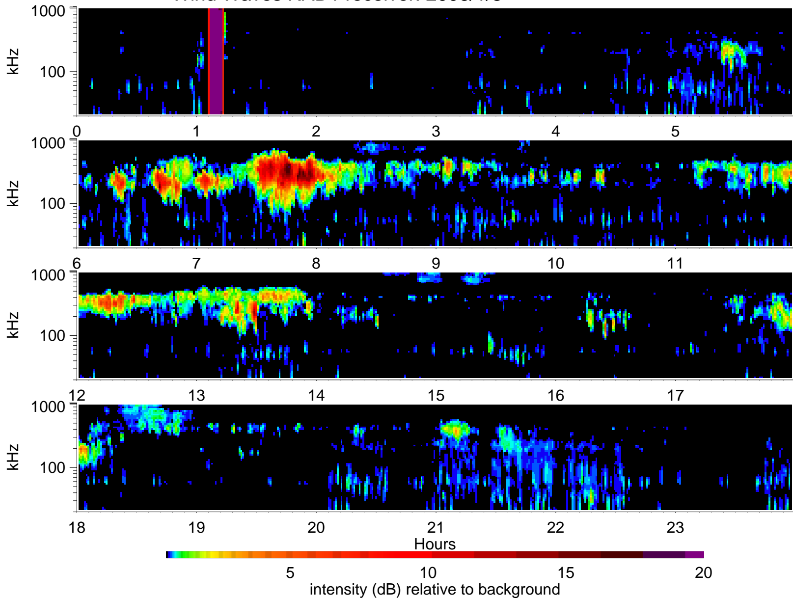
Wind Waves RAD1 receiver: 2006/1/8
