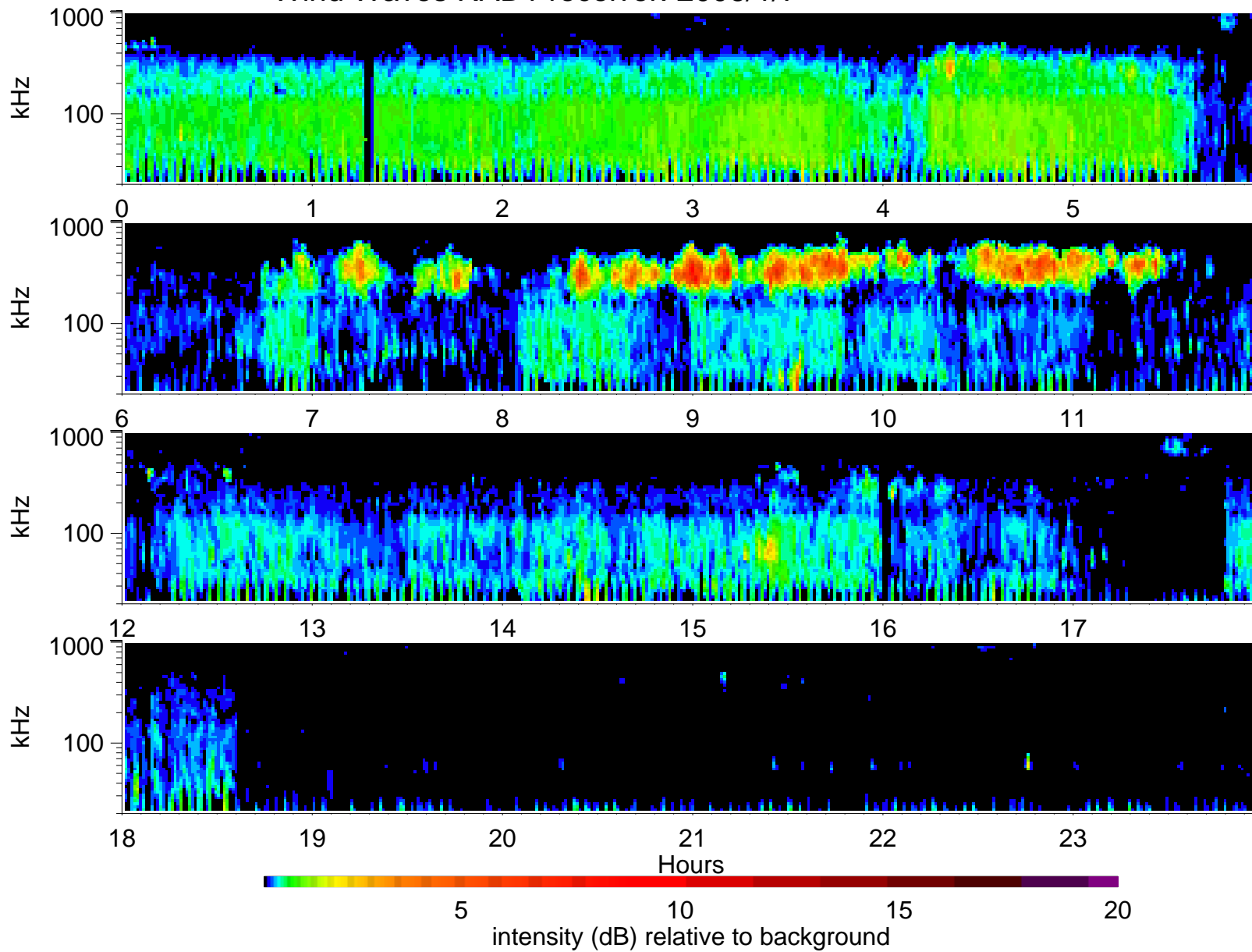
Wind Waves RAD1 receiver: 2006/1/7
